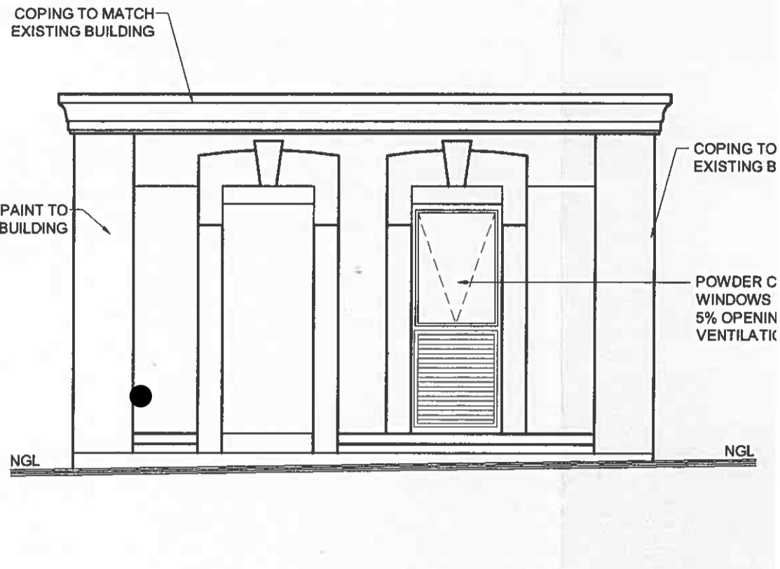
3 NORTH ELEVATION 400 SCALE 1:50 (A1) 1:100 (A3)
