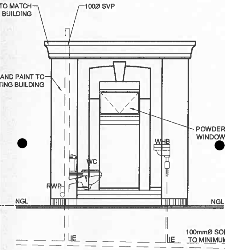
EAST ELEVATION SCALE 1:50 (A1) 1:100 (A3)
